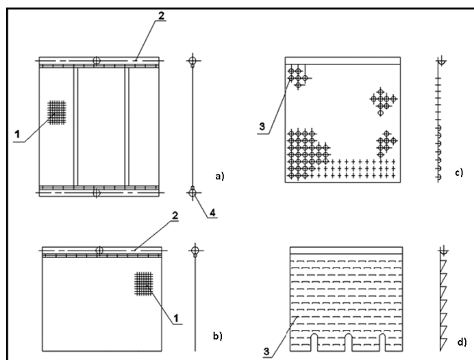
Figure 1 - Location of capillary-porous structures (a,b) and design realization of perforated plates (c, d): 1 – capillary-porous structures; 2 – feeding artery; 3 – perforated plates; 4 – water tray
